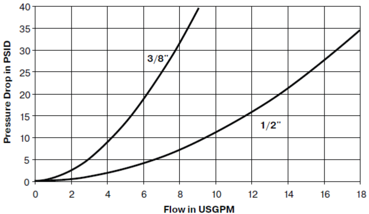
60 Series (3/8" & 1/2") Test Fluid: Oil - 150 SUS
