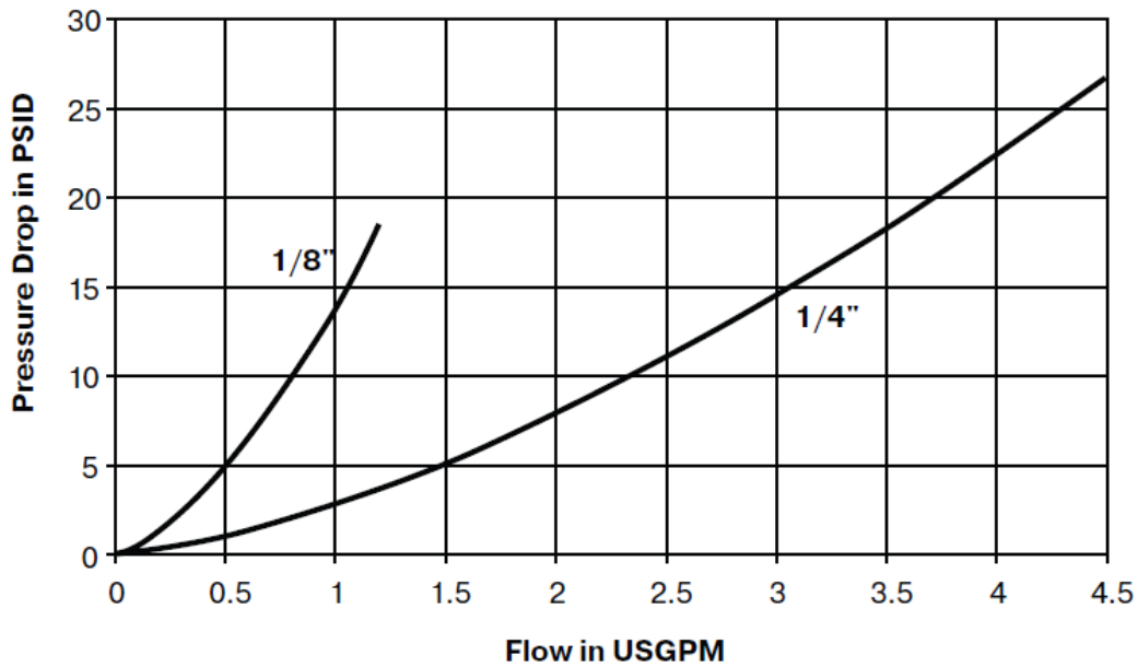
60 Series (1/8" & 1/4") Test Fluid: Oil - 150 SUS
