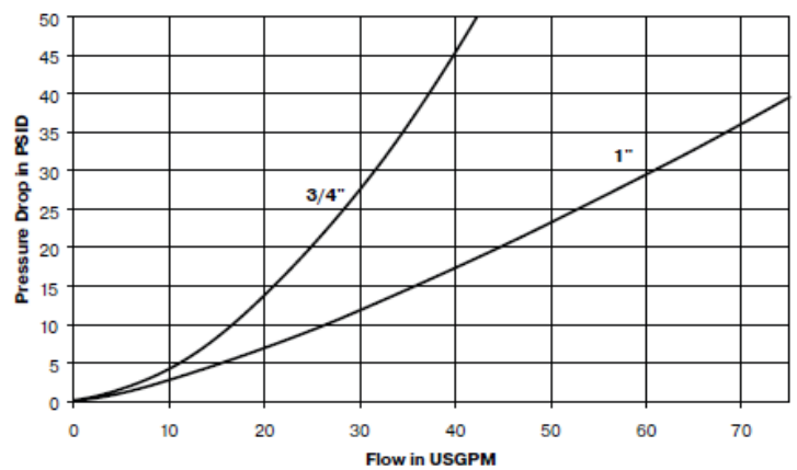
6600 Series (3/4" & 1") Test Fluid: Oil - 150 SUS
