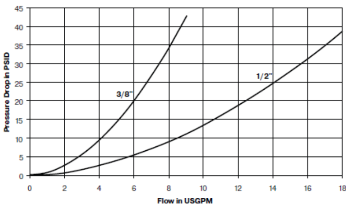
6600 Series (3/8" & 1/2") Test Fluid: Oil - 150 SUS
