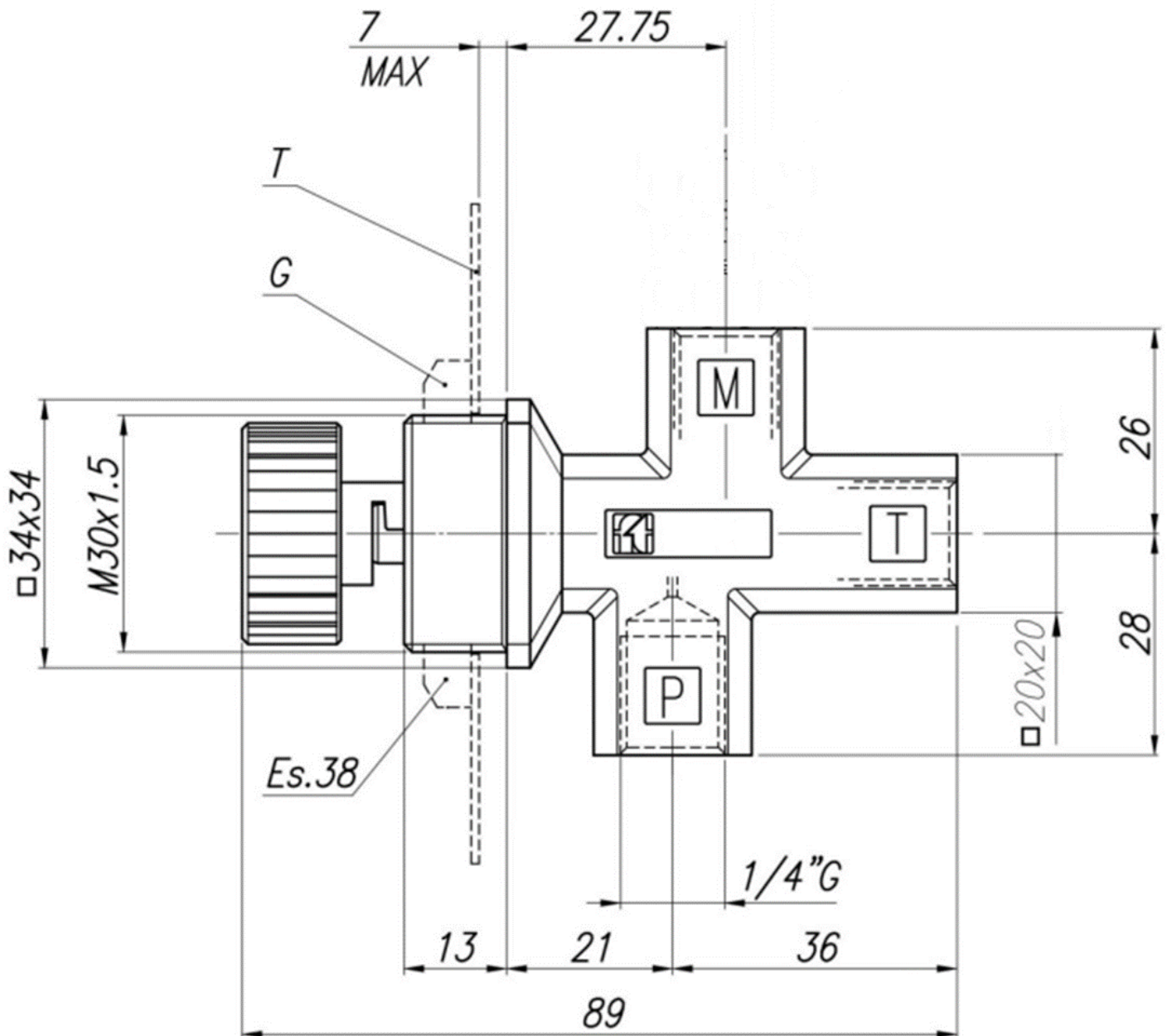
Dimension Drawing:
