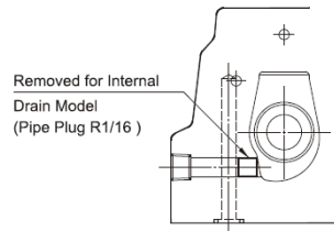
Section Y-Y
