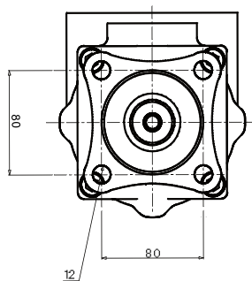
ODF Double Vane Pump Dimensions in mm
