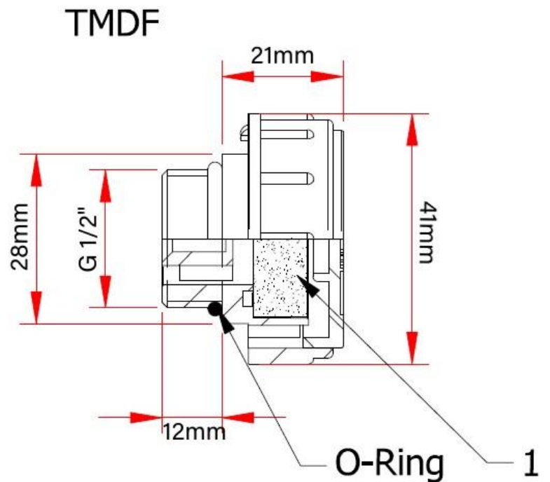
Polyurethane Air Filter
