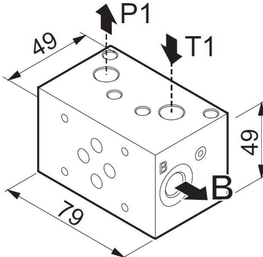
Installation Dimensions
