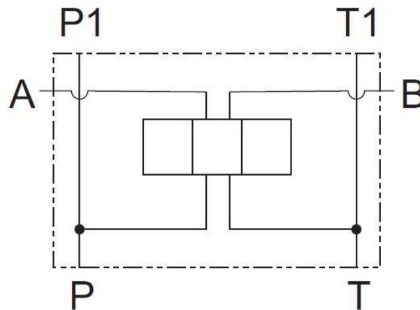
Symbol Drawing
