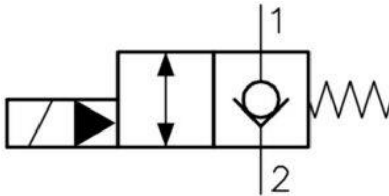
Symbol Drawing
