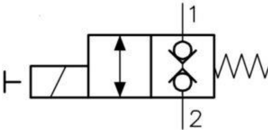
Symbol Drawing
